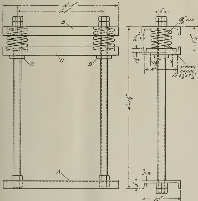
TESTING MACHINE FOR HYDRAULIC JACKS.
